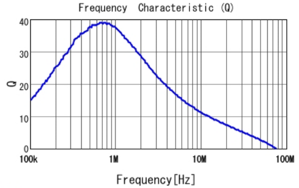
■ 1277AS-H-1R0M Q
