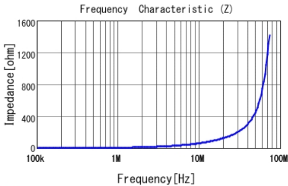
■ 1277AS-H-1R0M |Z|
