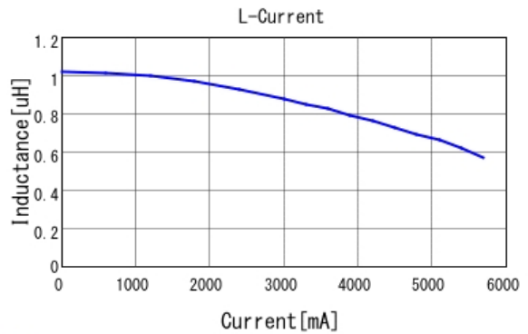
■ 1277AS-H-1R0M L-Current 20degC
