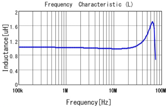
■ 1277AS-H-1R0M L
